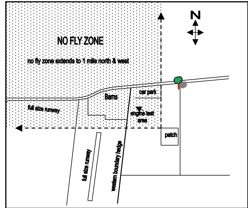
Figure 1 Landmead Flying Field Layout
